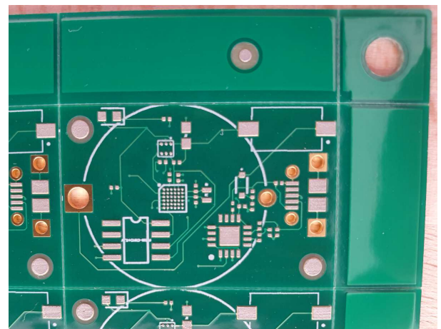
printing results for µBGA and 0201
